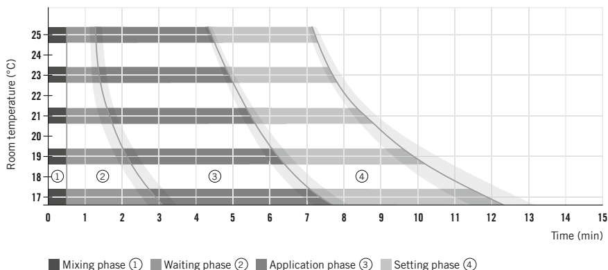
Working times of PALACOS® MV+G pro (not pre-chilled)
